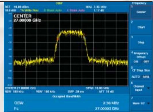
OBW measurement
