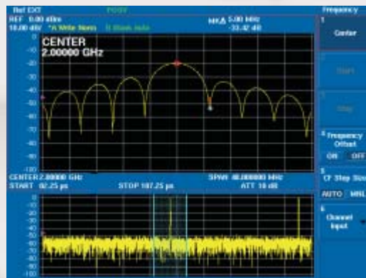
Radar wave measurement (OPT.55 for Wide-band time-domain analysis)
