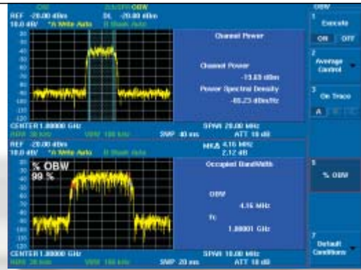
Simultaneous measurement of Cannel Power and OBW
